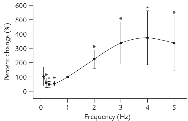
Figure 4. Plot of frequency-response of pulmonary vein (PV) sleeve contraction. The PV ring preparation was driven by electrical stimuli from the LA free wall and superfused with normal Tyrode solution. Frequency of electrical stimuli ranged from 0.1 Hz to 5 Hz. Data are expressed as mean \pm standard deviation. * p < 0.05 vs. value at 1 Hz (as a control, 100%).
