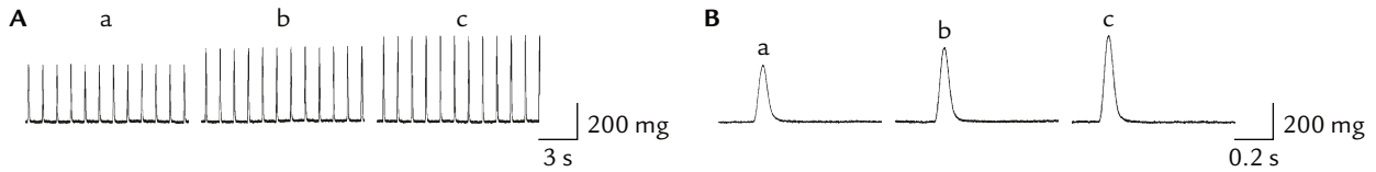
Figure 2. Effect of high external calcium on pulmonary vein (PV) sleeve contraction. The PV ring preparation was driven by 1 Hz of electrical stimuli from the LA free wall and superfused with normal Tyrode solution. (A) Slow sweep speed; (B) fast sweep speed. a = Ca 2.7 mM; b = Ca 5.4 mM; c = Ca 8.1 mM.
