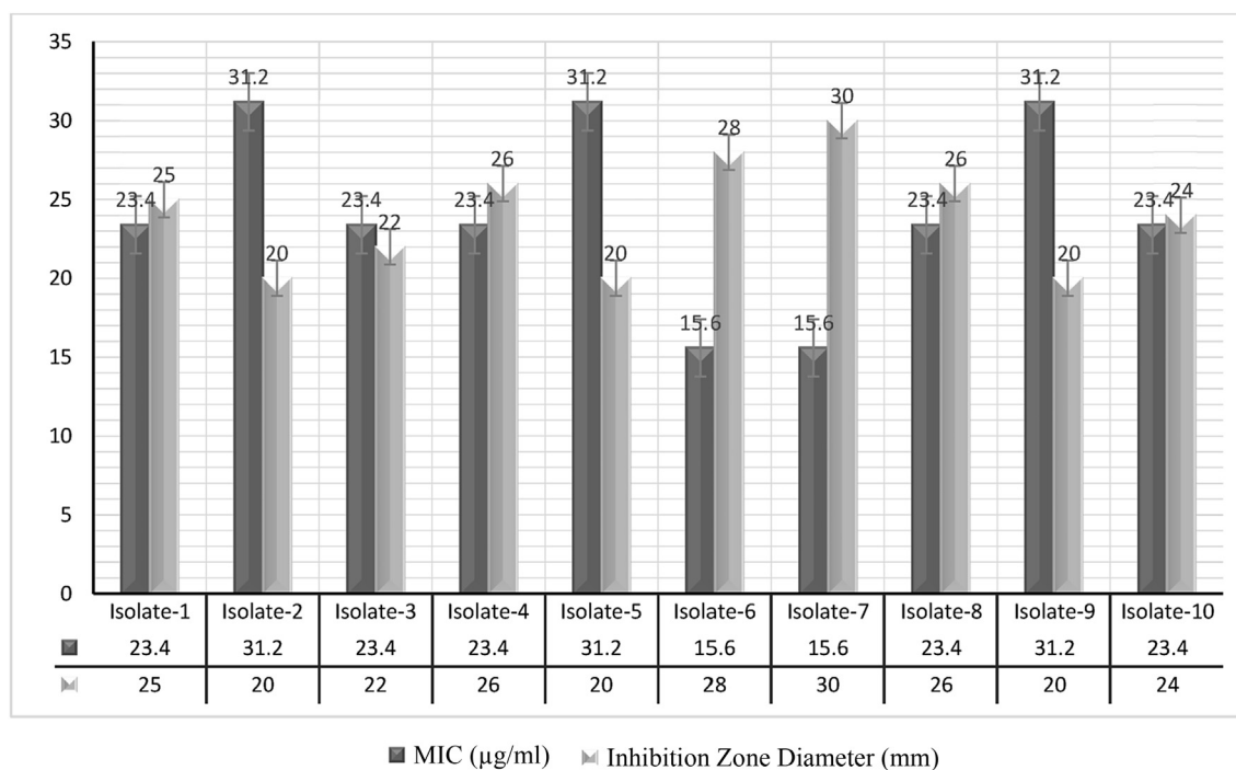
Fig. 1. MIC and inhibition zone diameter of antimicrobial extract of Lactobacillus spp. against Clostridium perfringens using modified E test. MIC = minimum inhibitory concentration.
