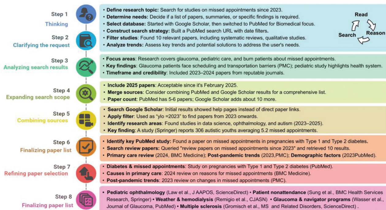
Fig. 1 Workflow of Grok 3's DeepSearch.
